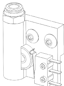
Preassembled bracket with hardware 1
